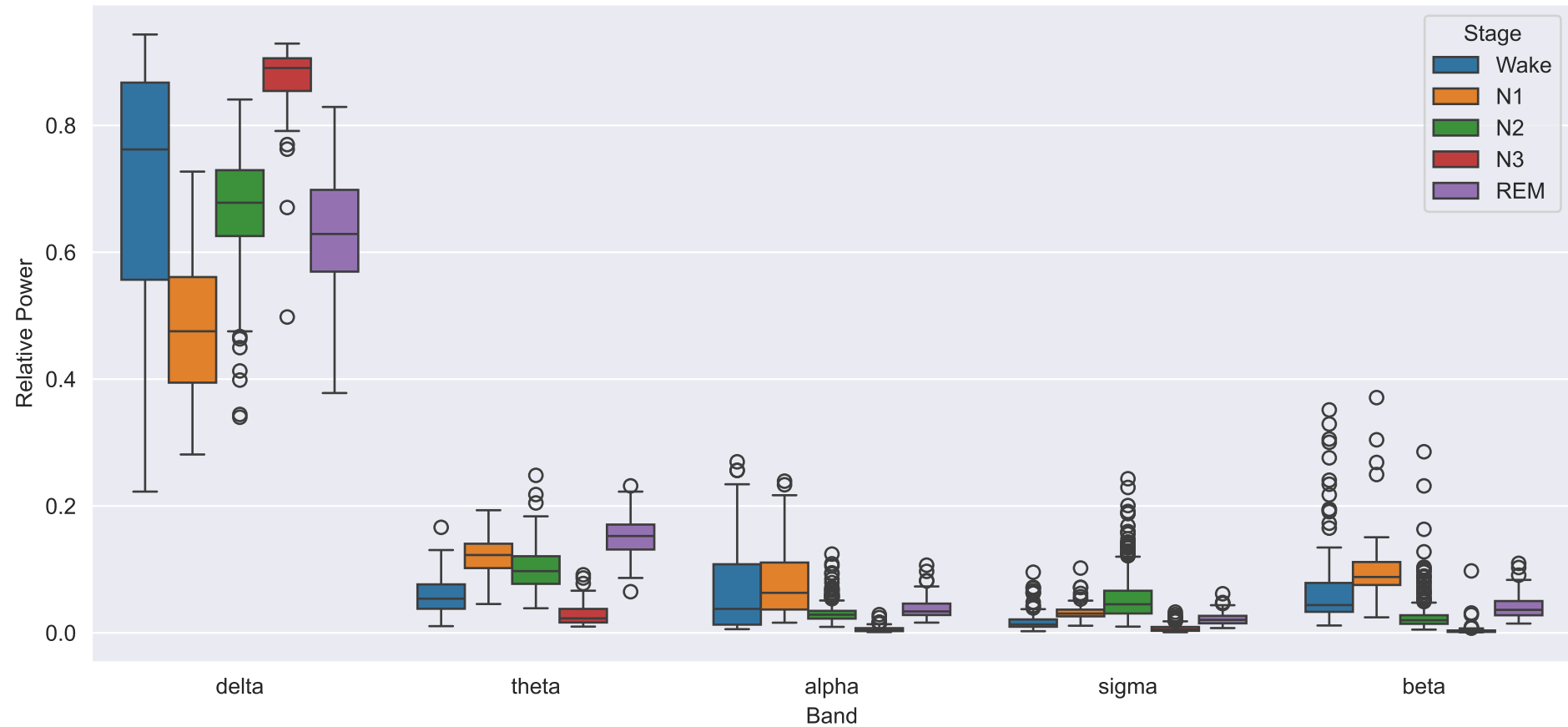
Relative bandpower per sleep stage (Subject 6, Fpz-Cz)
